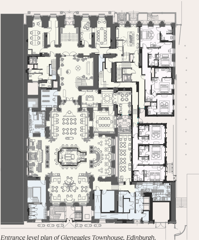
Entrance level plan of Gleneagles Townhouse, Edinburgh.
