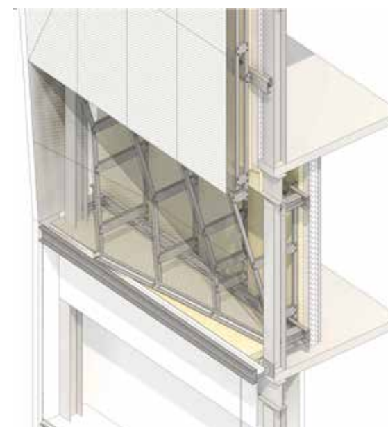
Facade detail.
