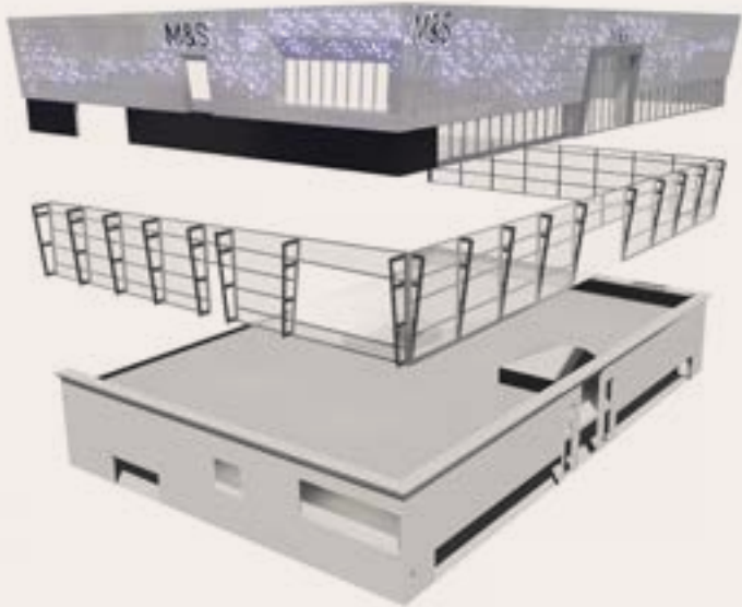
Facade exploded axonometric.
